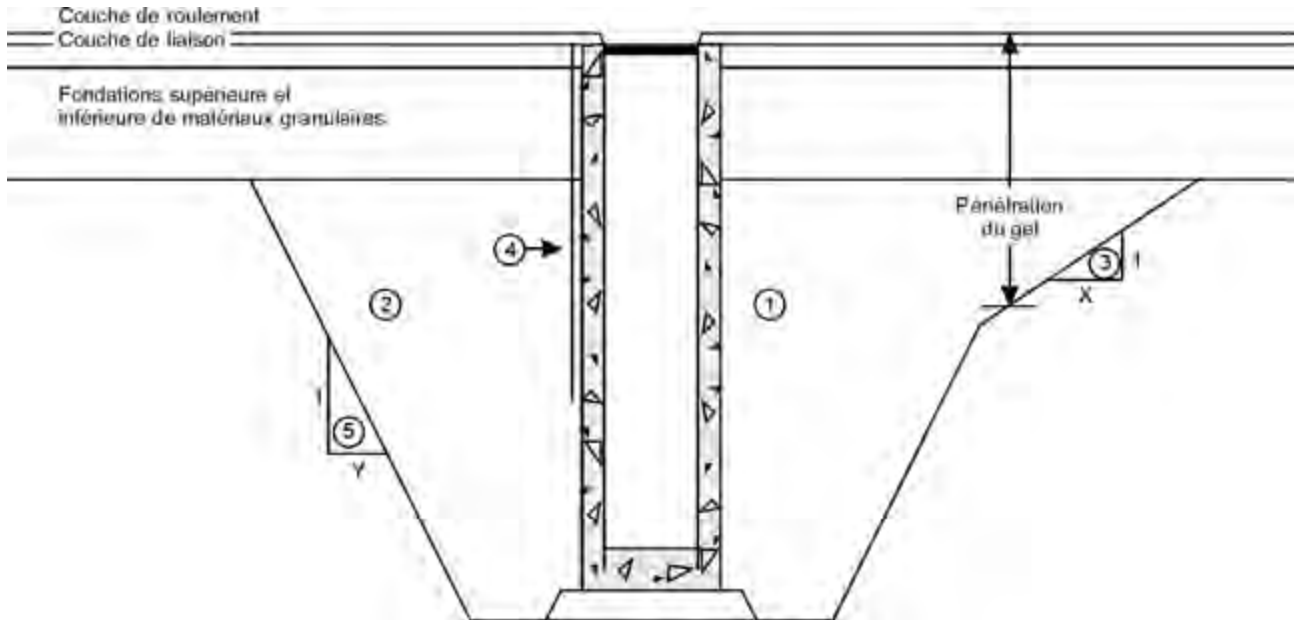
Figure 3-3 : Devis de construction.
